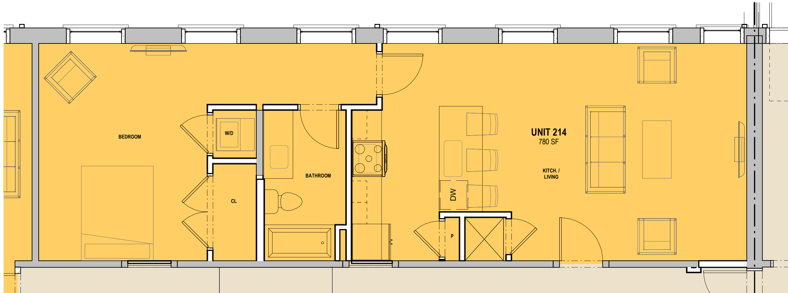
1 LEVEL 02 - UNIT 214 U2.14 SCALE: 1/4" = 1'-0"
