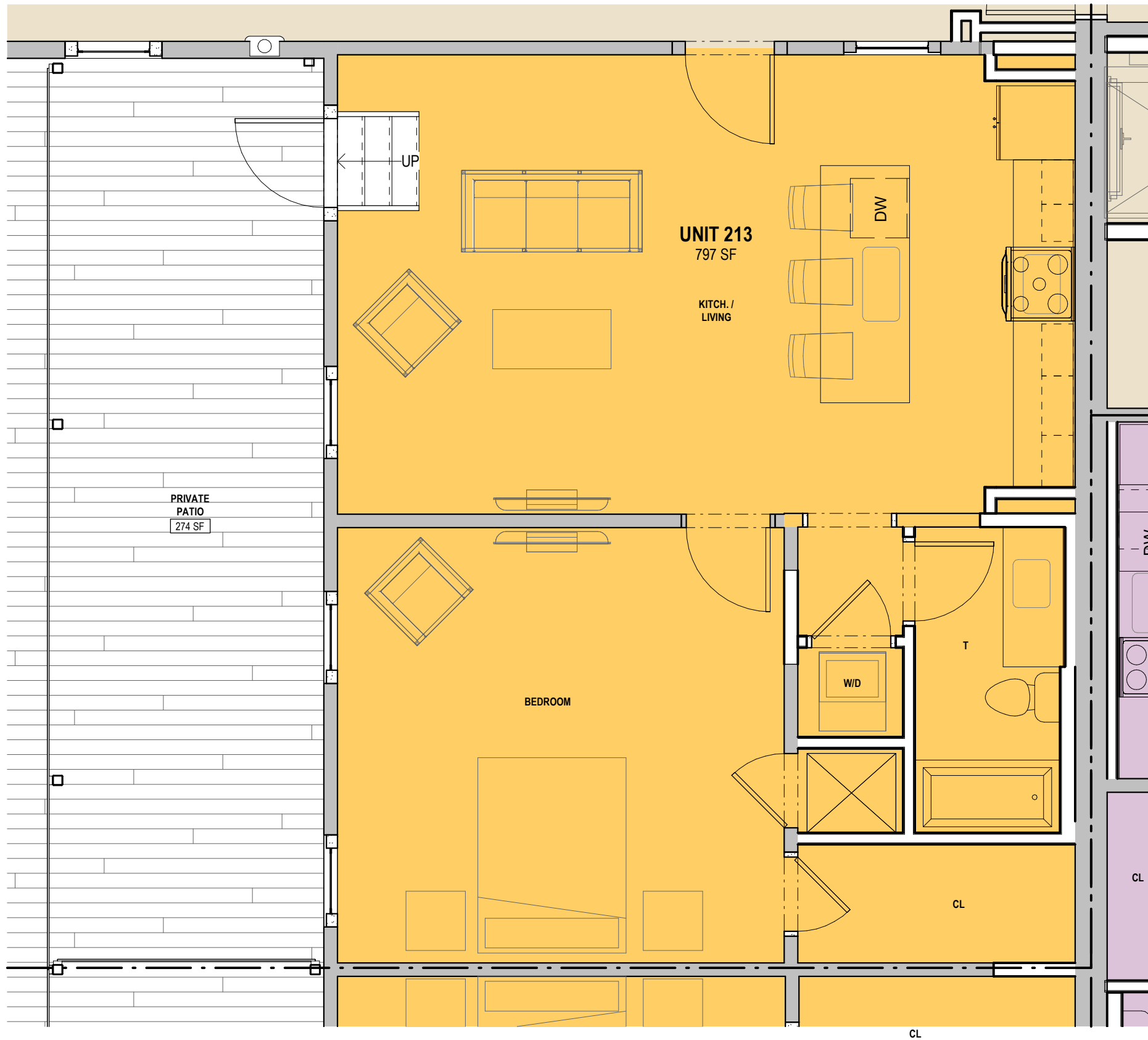
1 LEVEL 02 - UNIT 213 U2.13 SCALE: 1/4" = 1'-0"
