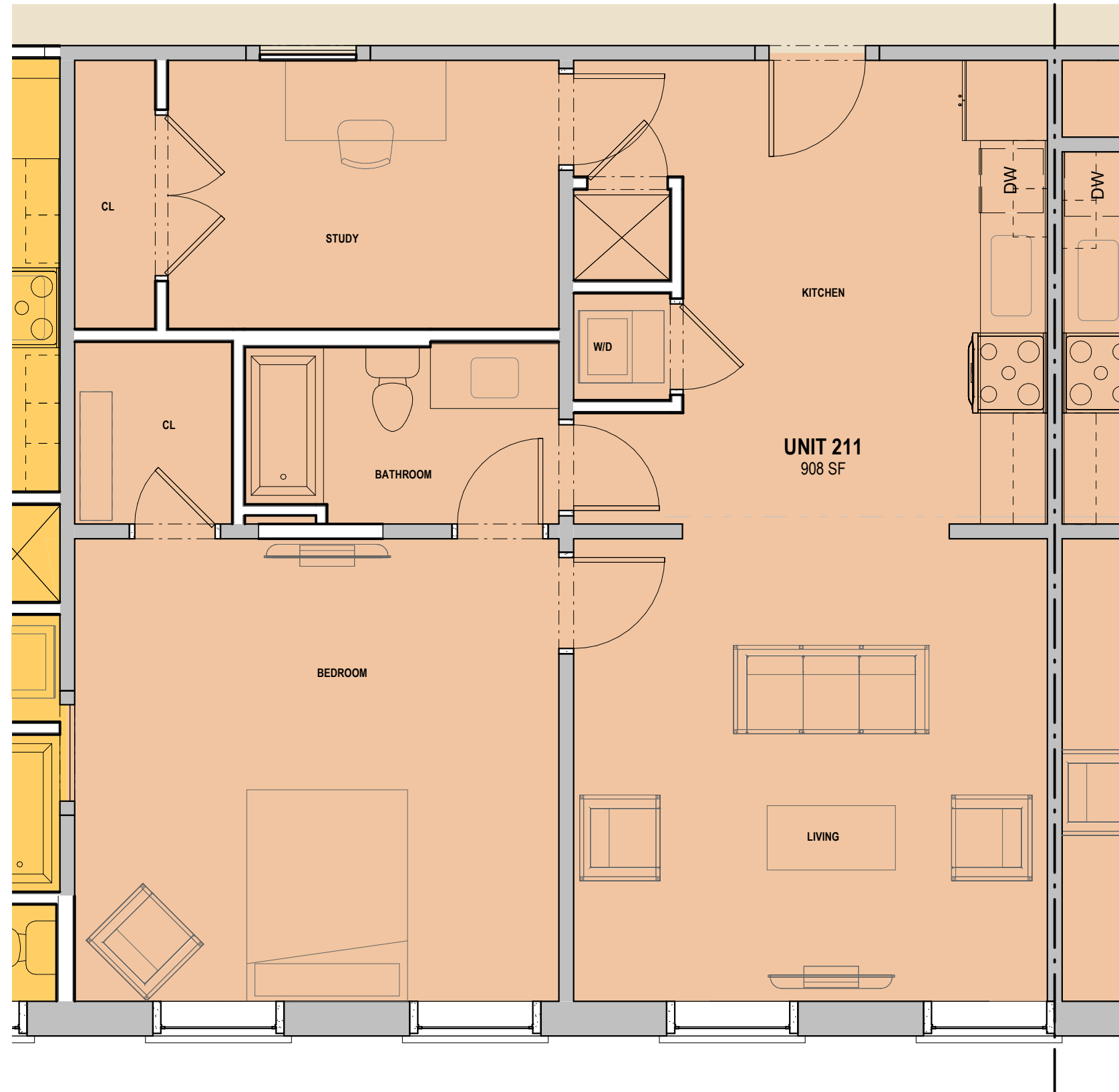
1 LEVEL 02 - UNIT 211 U2.11 SCALE: 1/4" = 1'-0"
