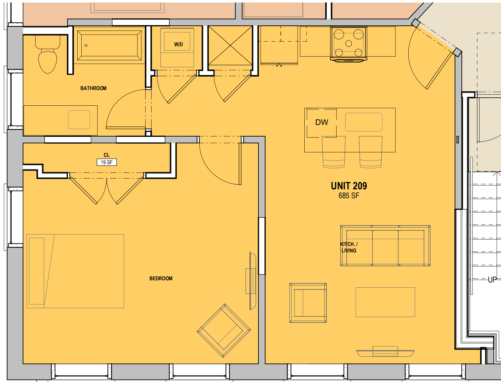
1 LEVEL 02 - UNIT 209 U2.09 SCALE: 1/4" = 1'-0"
