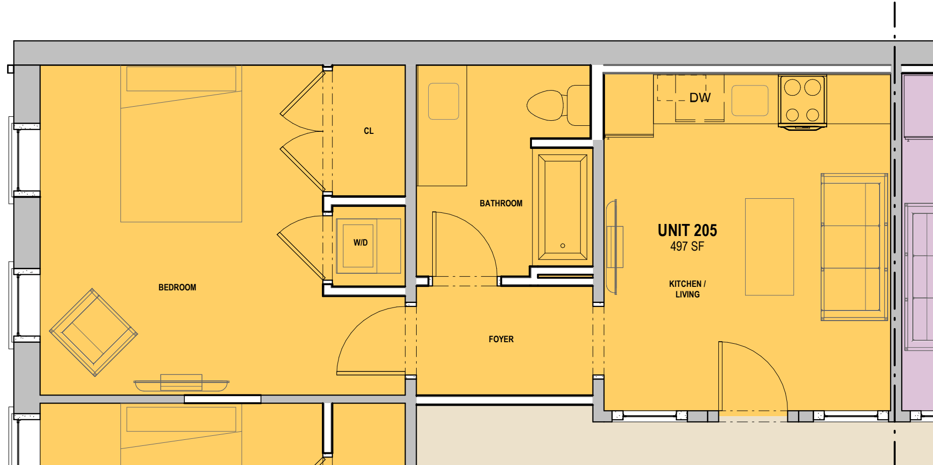
1 LEVEL 02 - UNIT 205 U2.05 SCALE: 1/4" = 1'-0"
