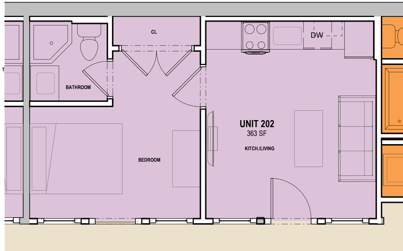
1 LEVEL 02 - UNIT 202 U2.02 SCALE: 1/4" = 1'-0"
